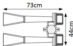
Speaker array top view
